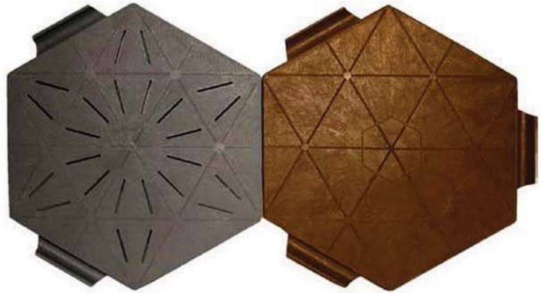
Eco slabs are available in both solid as well as slotted for additional drainage. Available in both grey and brown colours.
